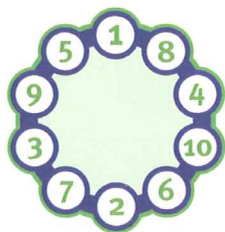
Wheel nut tightening sequence
